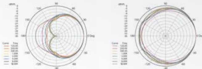
Polar Chart
