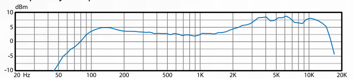
Frequency Response
