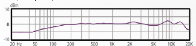
Frequency Response
