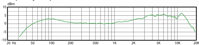
Frequency Response
