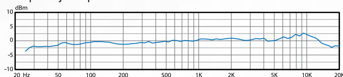
Frequency Response
