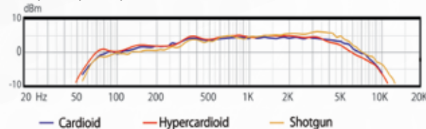
Frequency Response
