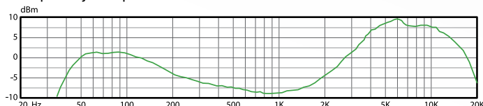
Frequency Response
