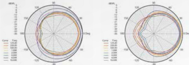
Polar Chart
