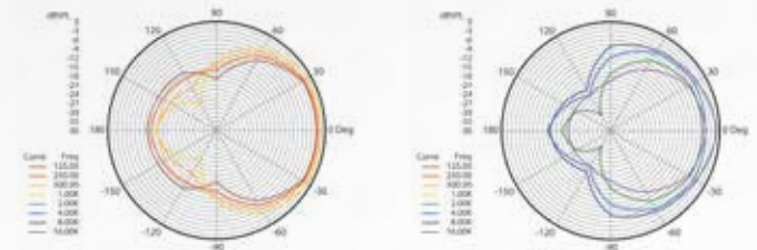
Polar Chart
