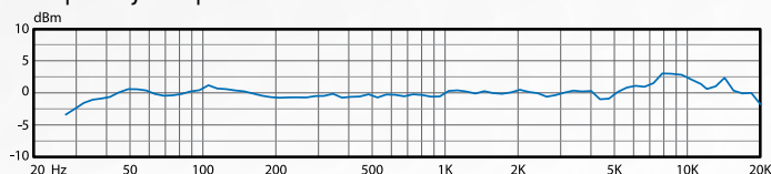
Frequency Response
